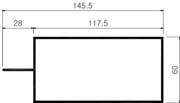
K A T - 2 5 0 2 1.84 kg/m, 1.8T
