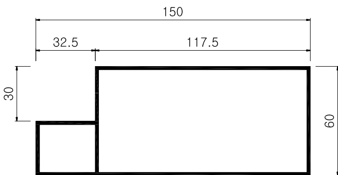
K A T - 2 5 0 6 2.16 kg/m, 1.8T
