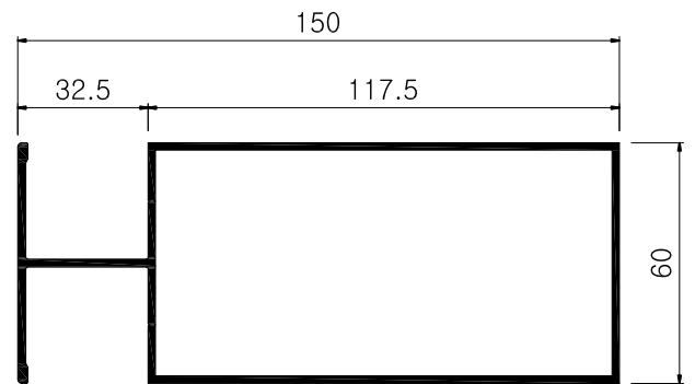
K A T - 2 5 0 5 2.19 kg/m, 1.8T
