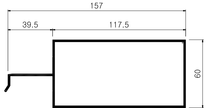
K A T - 2 5 0 3 1.97 kg/m, 1.8T
