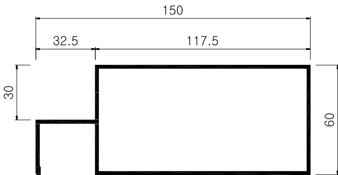
K A T - 2 5 0 4 2.02 kg/m, 1.8T
