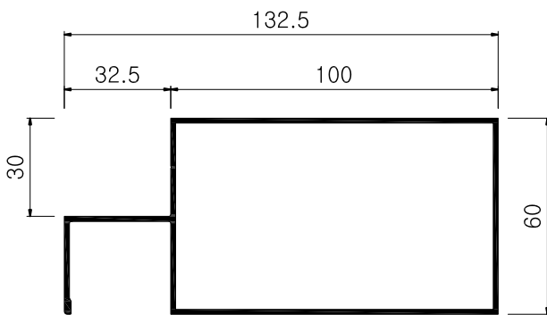
K A T - 1 3 0 4 1.54 kg/m, 1.5T
