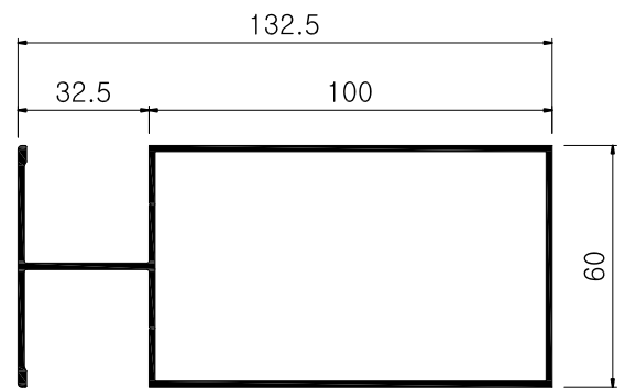
K A T - 1 3 0 5 1.67 kg/m, 1.5T
