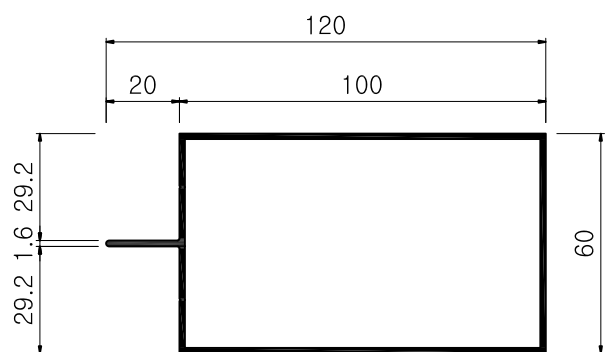
K A T - 1 3 0 2 ~ 1 1.36 kg/m, 1.5T
